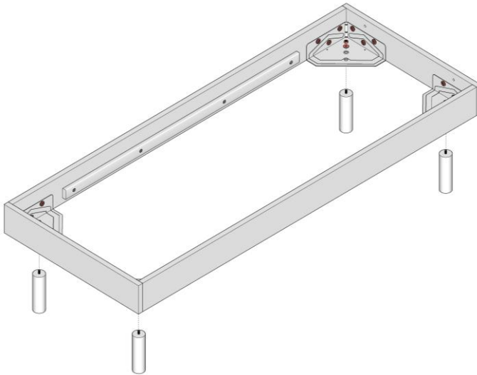
Fit all four legs
