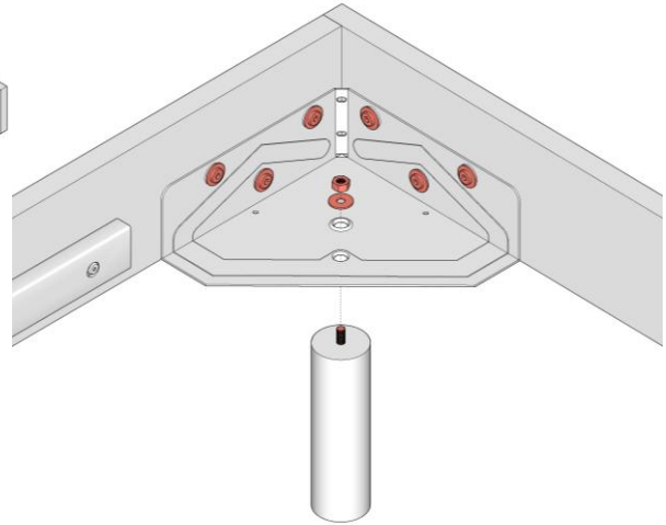
Leg fixing detail
