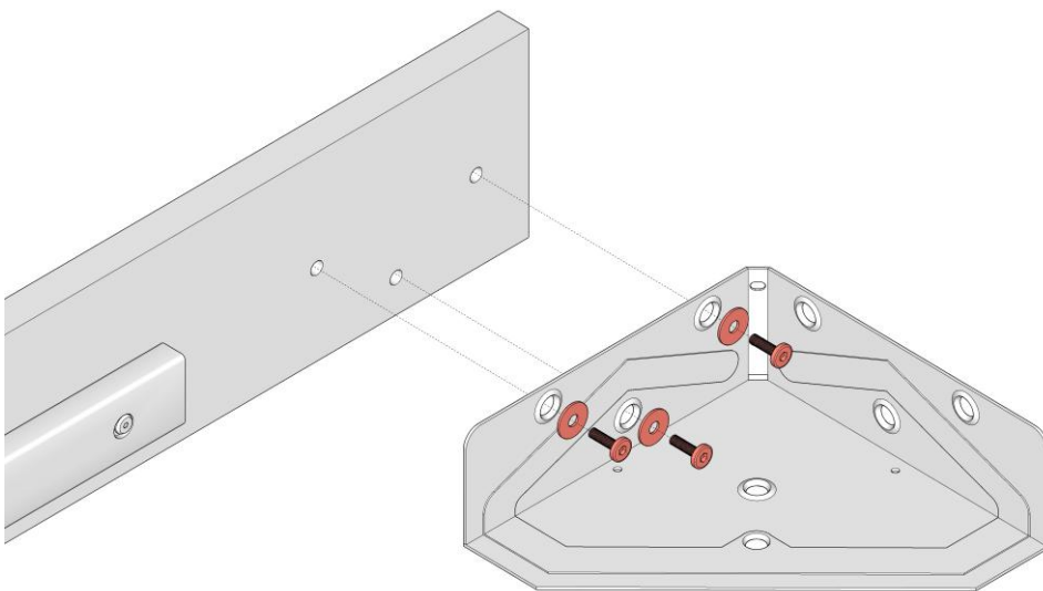
Corner bracket detail with three bolts and washers
