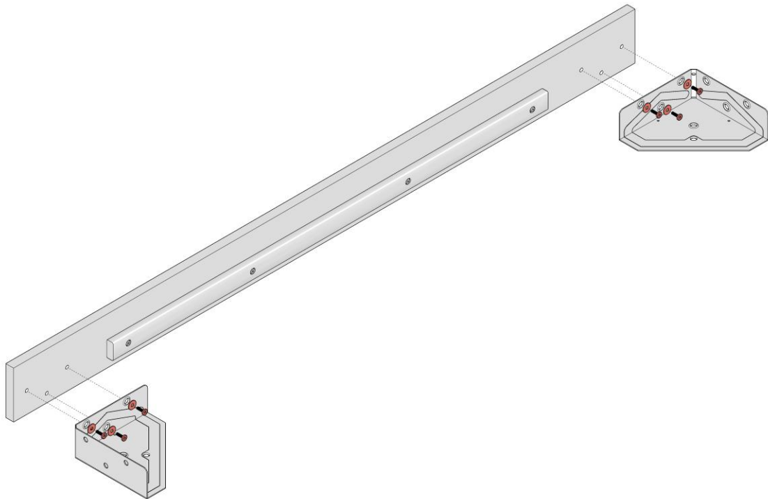
Fit two brackets to each side rail
